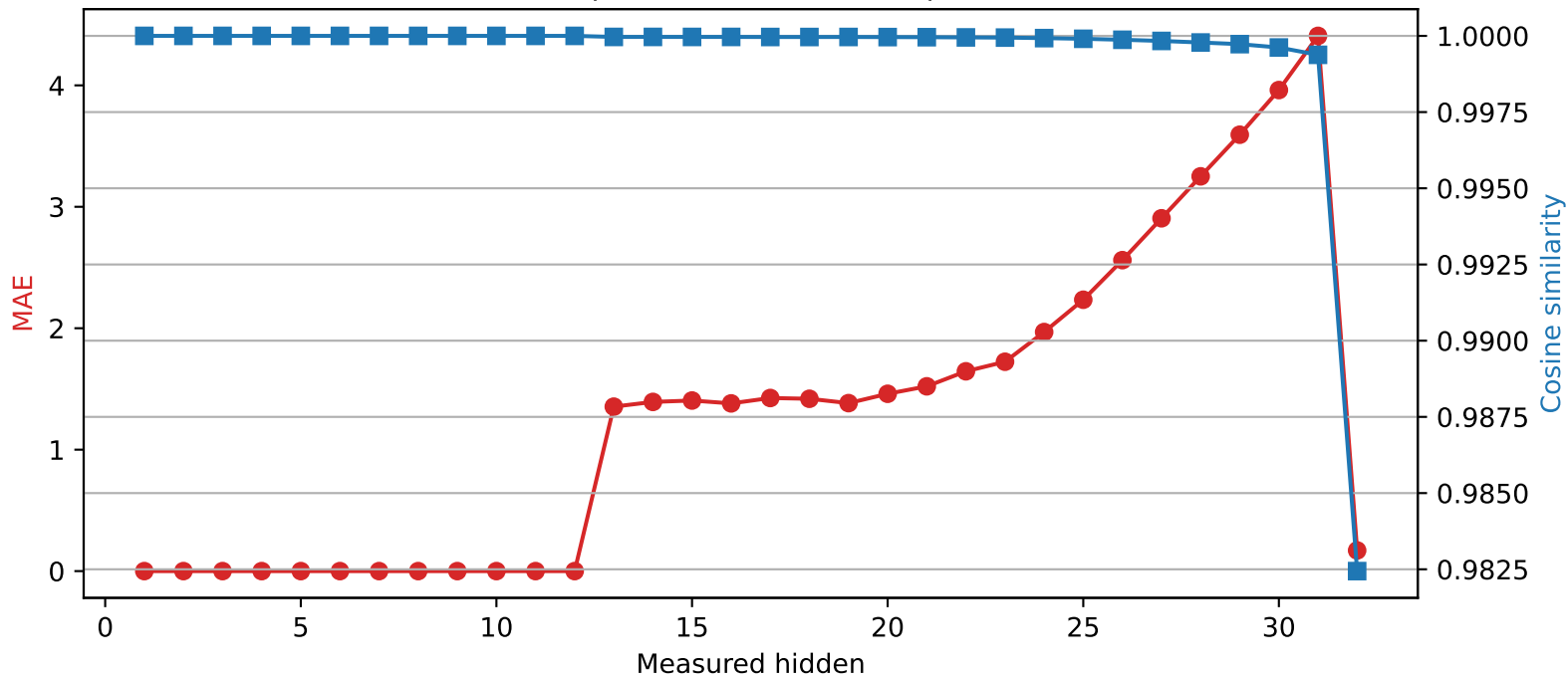
SmolLM2-360M | Quantized layer 12 | float16 \rightarrow int4
