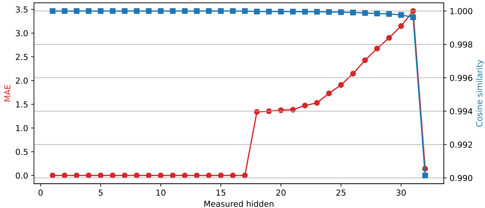
SmolLM2-360M | Quantized layer 17 | float16 \rightarrow int4
