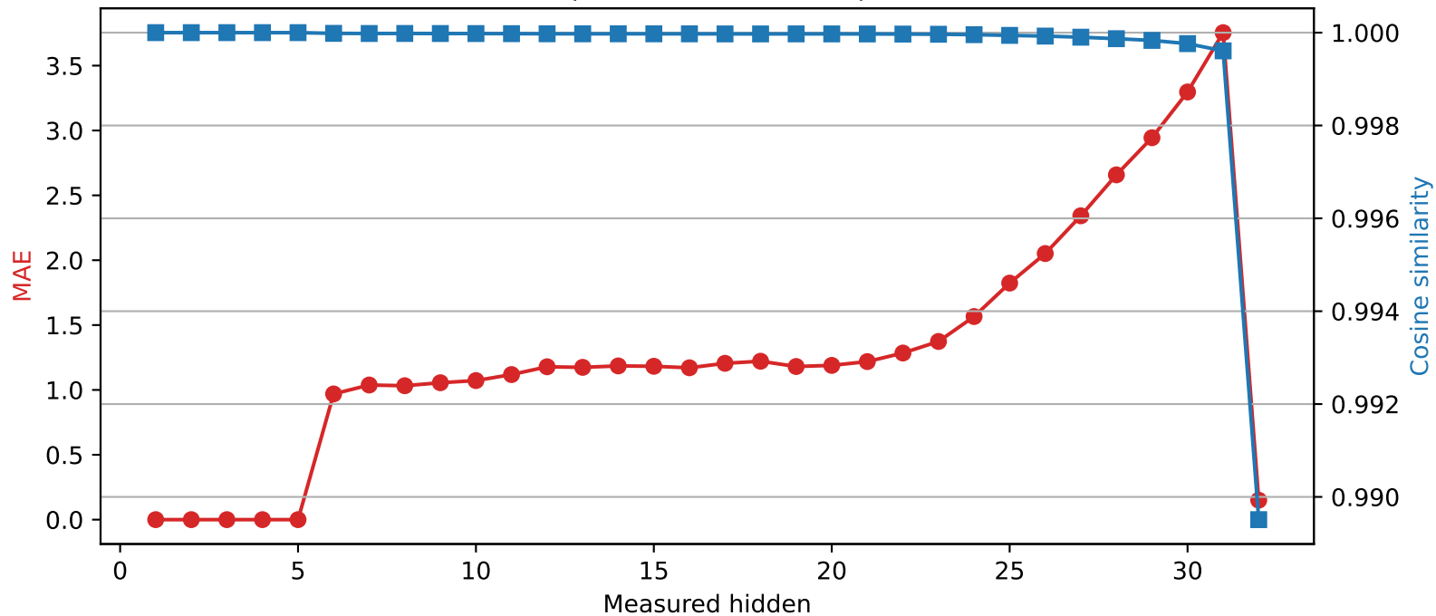
SmolLM2-360M | Quantized layer 5 | float16 \rightarrow int4
