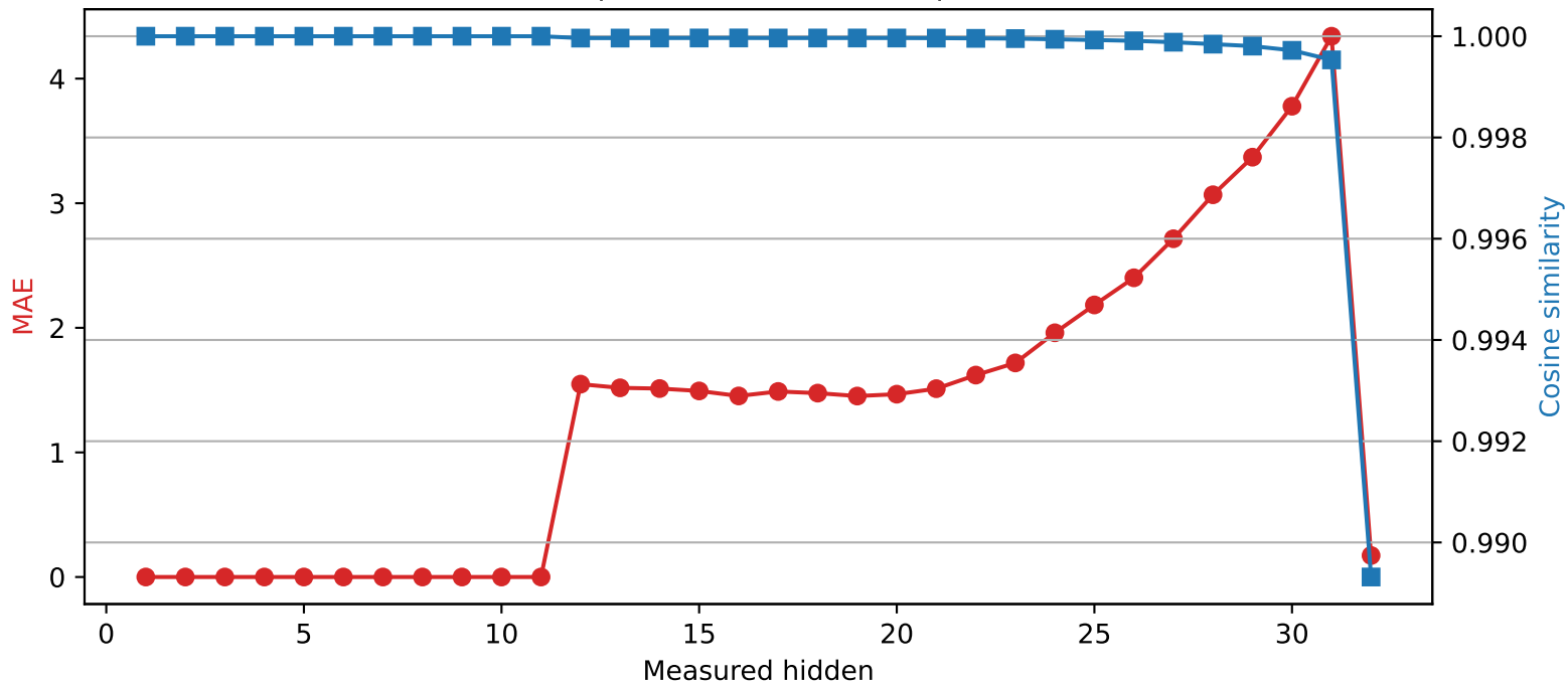
SmolLM2-360M | Quantized layer 11 | float16 → int4
