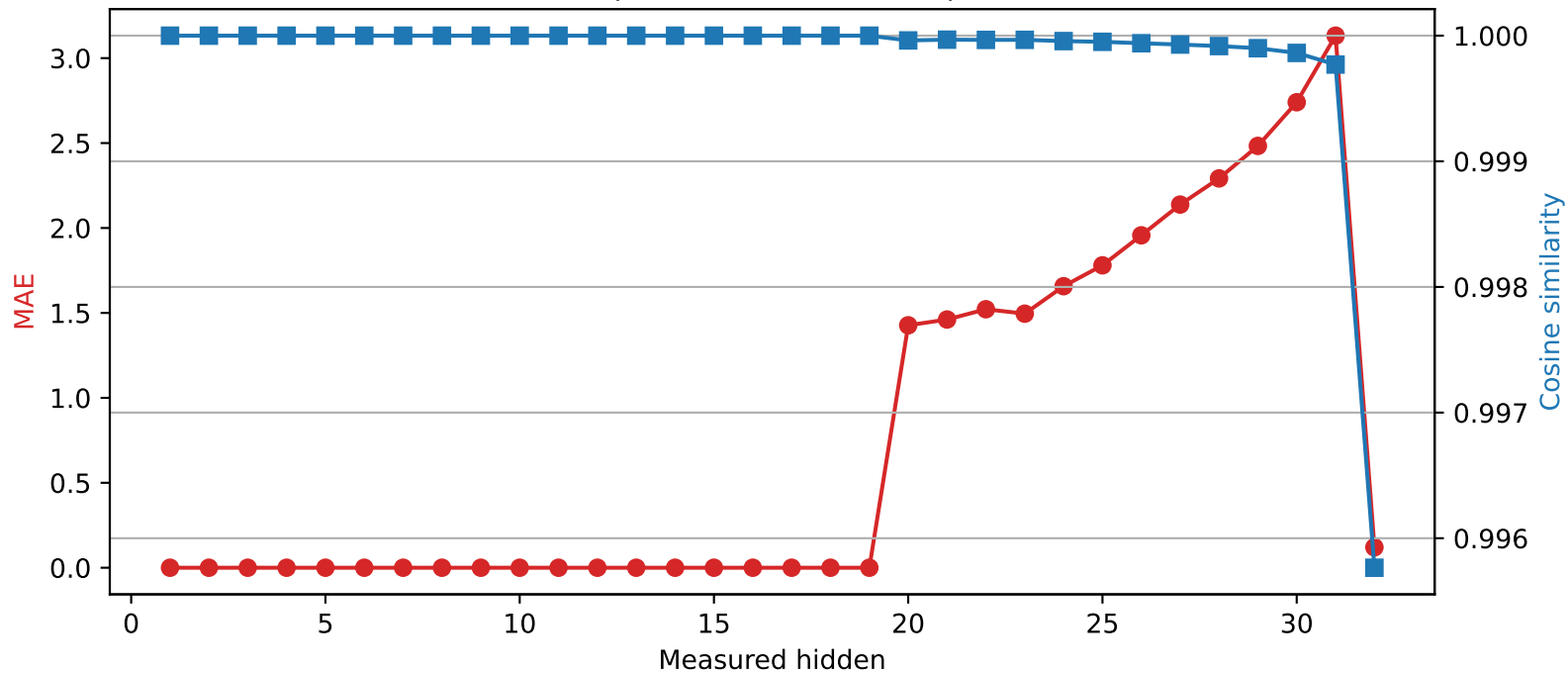
SmolLM2-360M | Quantized layer 19 | float16 \rightarrow int4
