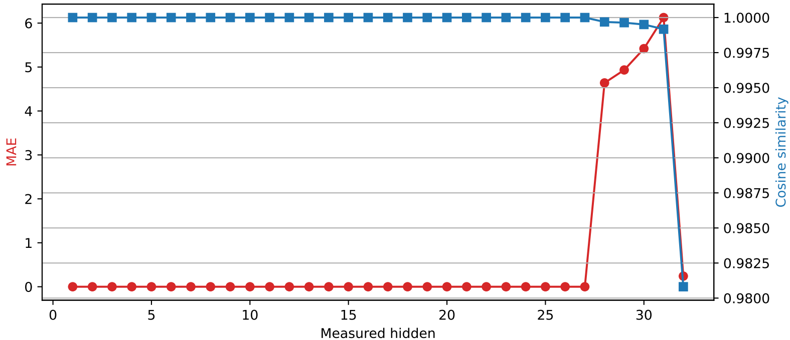
SmolLM2-360M | Quantized layer 27 | float16 → int4
