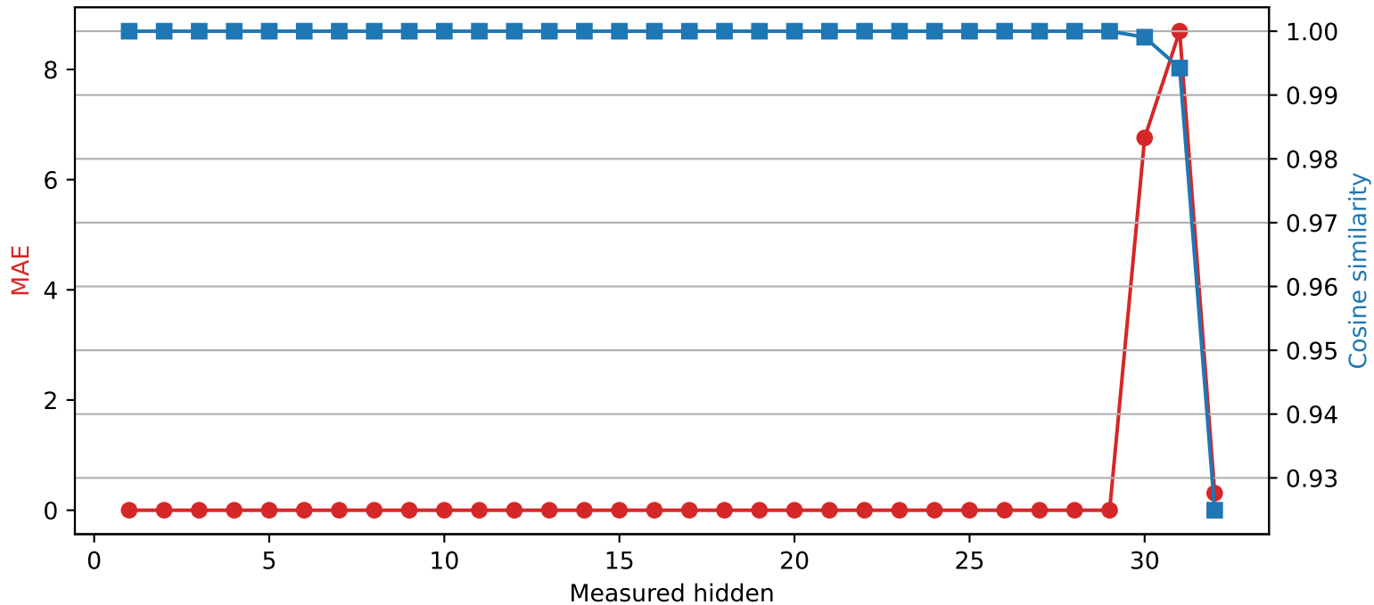
SmolLM2-360M | Quantized layer 29 | float16 → int4
