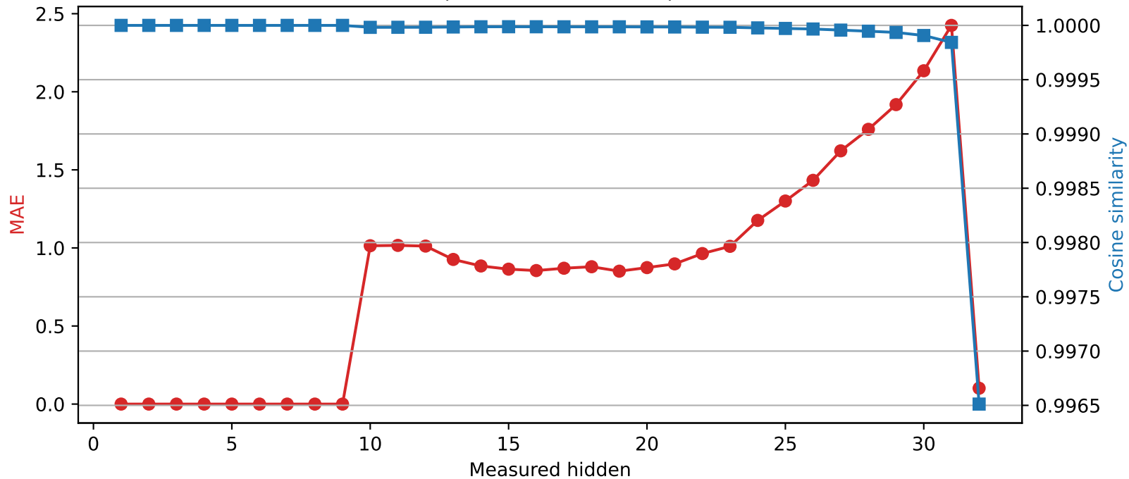
SmolLM2-360M | Quantized layer 9 | float16 → int4
