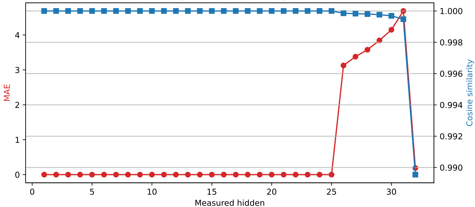
SmolLM2-360M | Quantized layer 25 | float16 \rightarrow int4
