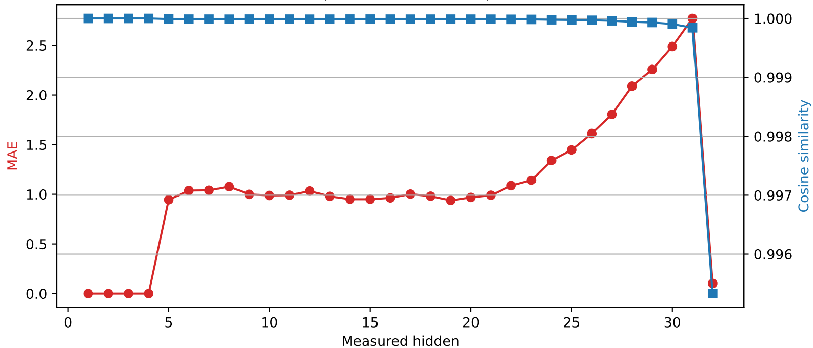
SmolLM2-360M | Quantized layer 4 | float16 \rightarrow int4
