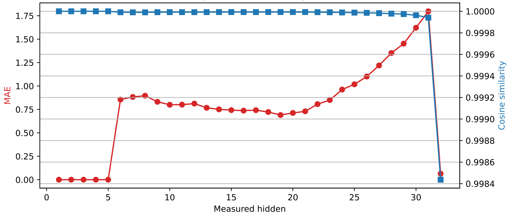
SmolLM2-360M | Quantized layer 5 | float16 → int4
