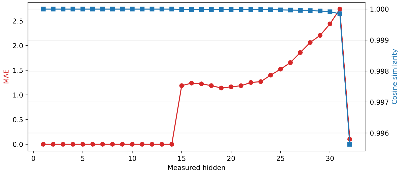
SmolLM2-360M | Quantized layer 14 | float16 \rightarrow int4
