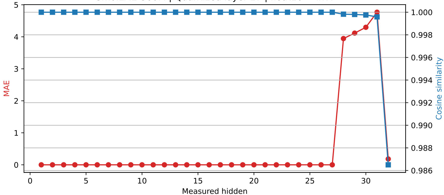
SmolLM2-360M | Quantized layer 27 | float16 \rightarrow int4
