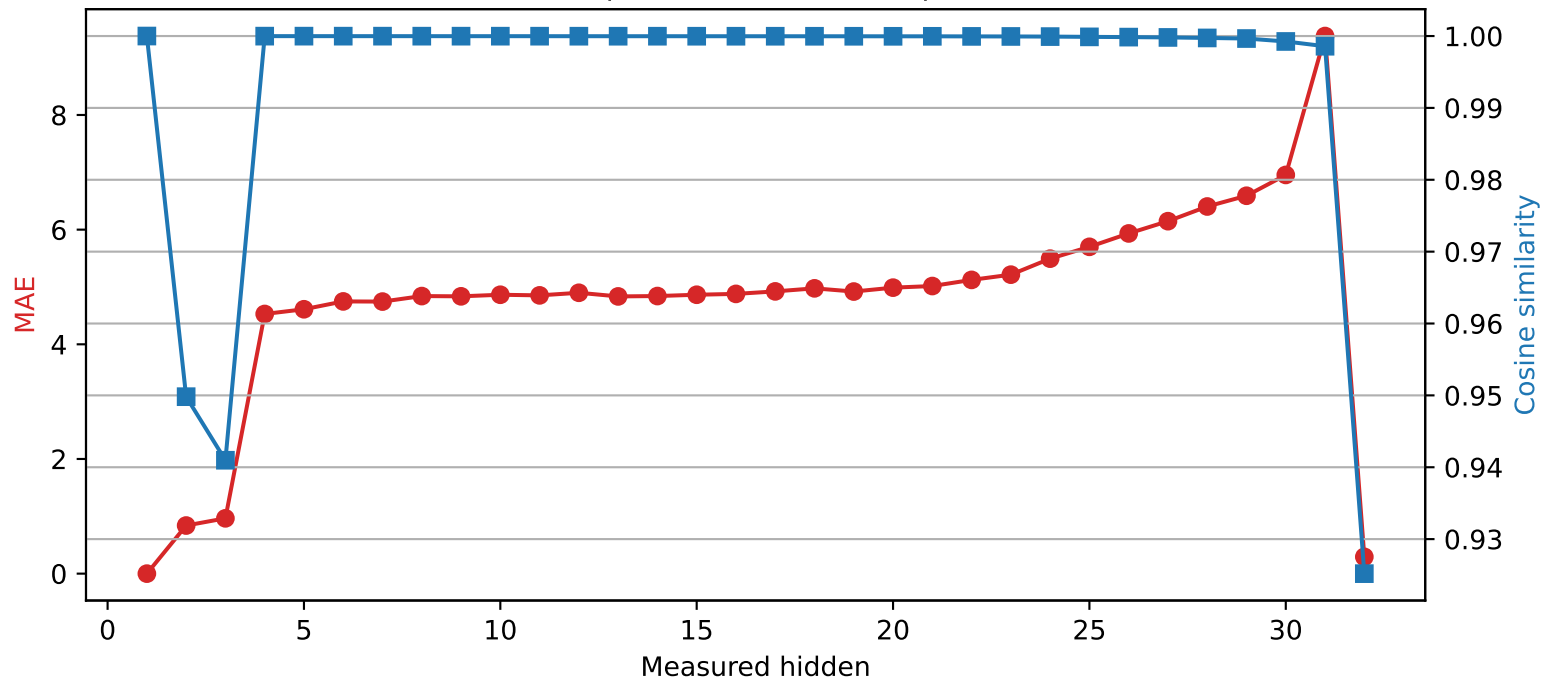
SmolLM2-360M | Quantized layer 1 | float32 \rightarrow int4
