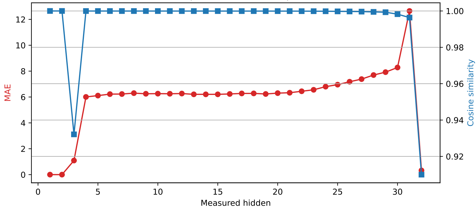
SmolLM2-360M | Quantized layer 2 | float32 → int4
