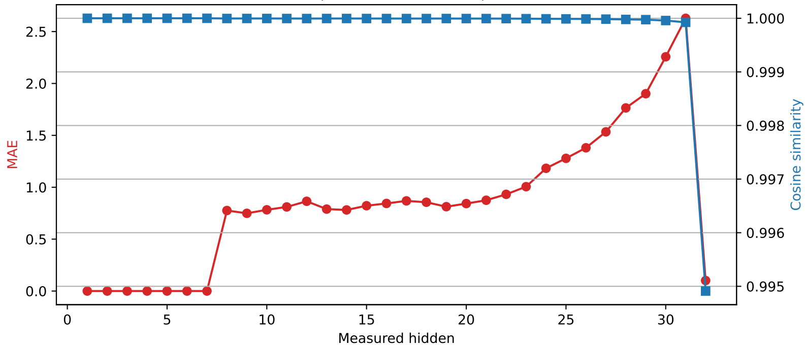
SmolLM2-360M | Quantized layer 7 | float32 \rightarrow int4
