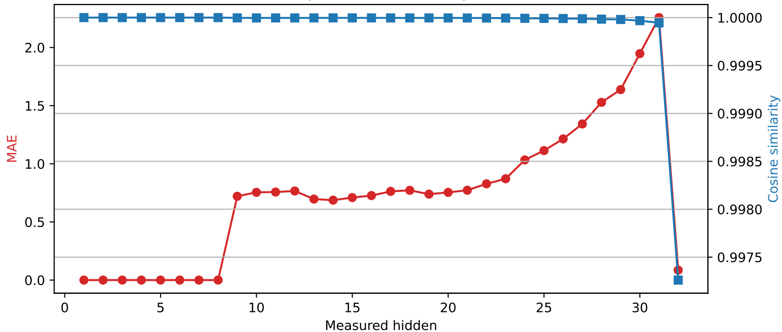
SmolLM2-360M | Quantized layer 8 | float32 \rightarrow int4
