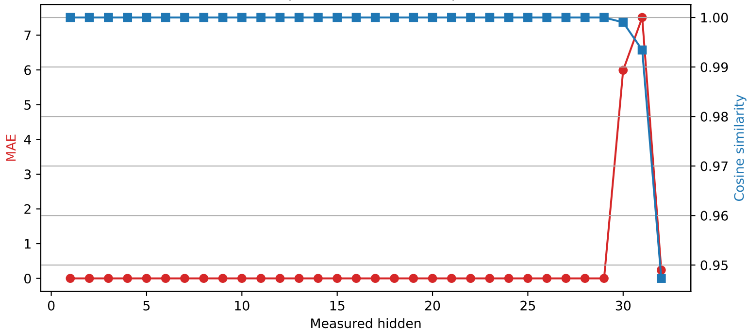
SmolLM2-360M | Quantized layer 29 | float32 → int4
