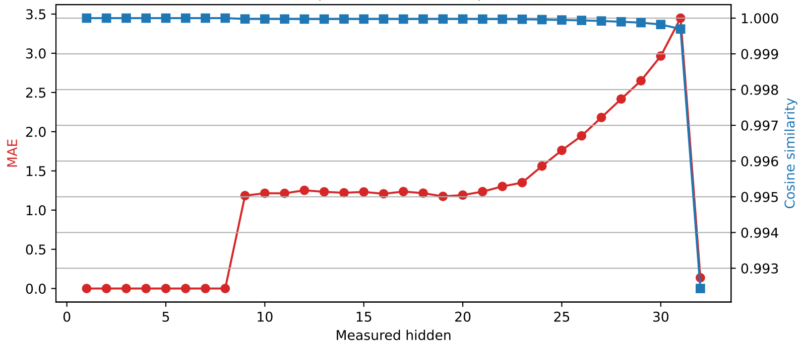
SmolLM2-360M | Quantized layer 8 | float32 → int4
