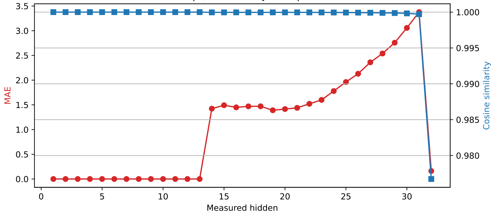
SmolLM2-360M | Quantized layer 13 | float32 → int4
