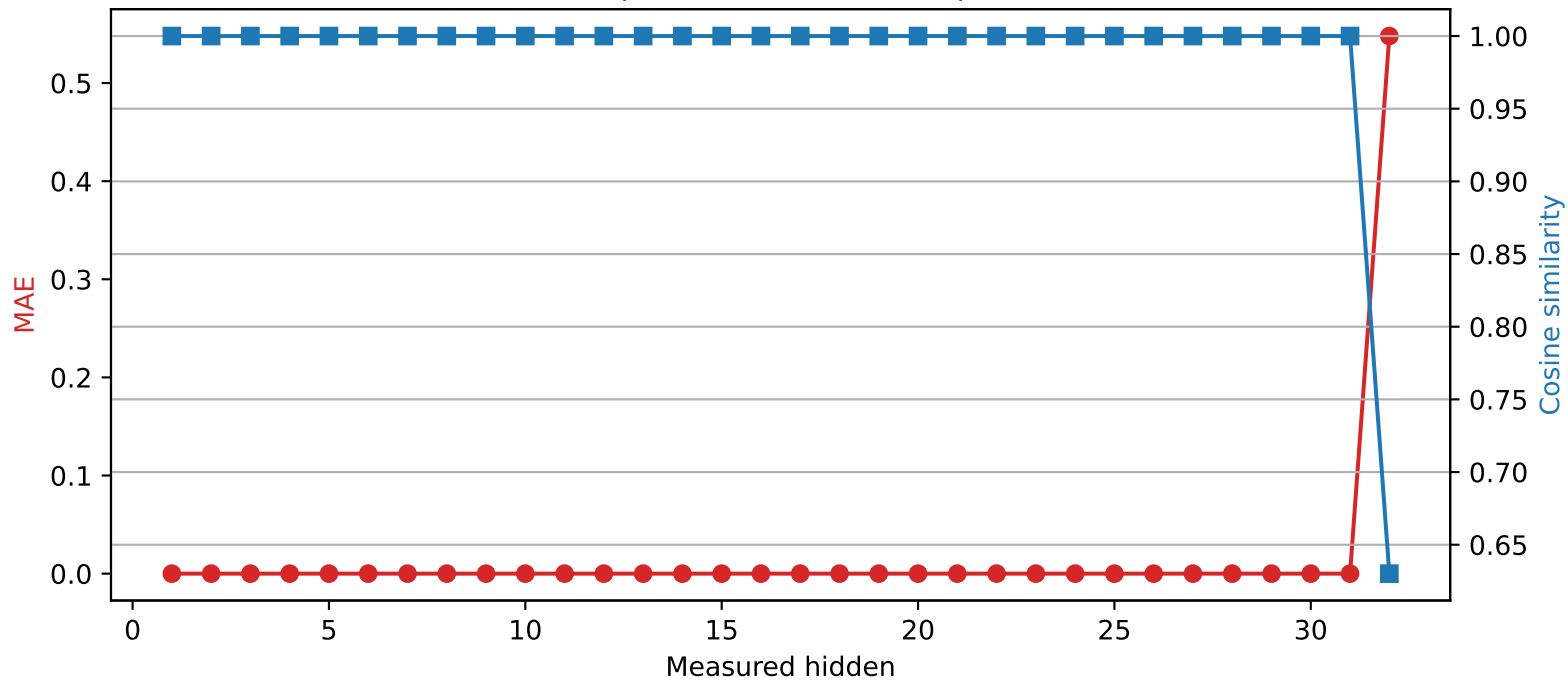
SmolLM2-360M | Quantized layer 31 | float32 → int4
