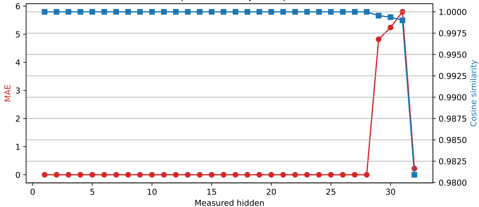
SmolLM2-360M | Quantized layer 28 | float64 → int4
