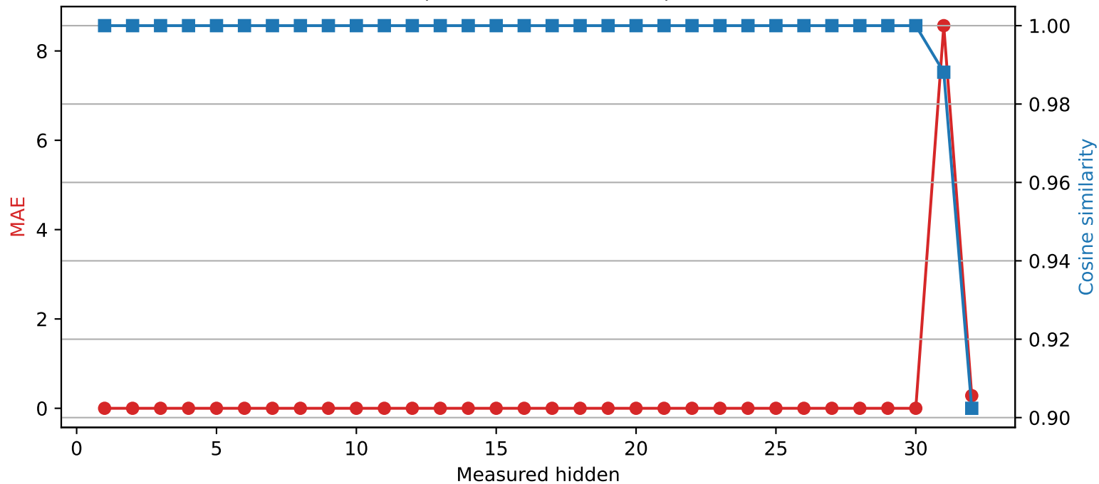
SmolLM2-360M | Quantized layer 30 | float64 → int4
