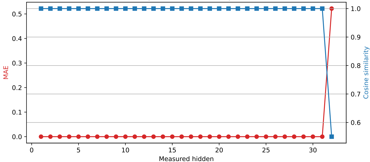
SmolLM2-360M | Quantized layer 31 | float64 → int4
