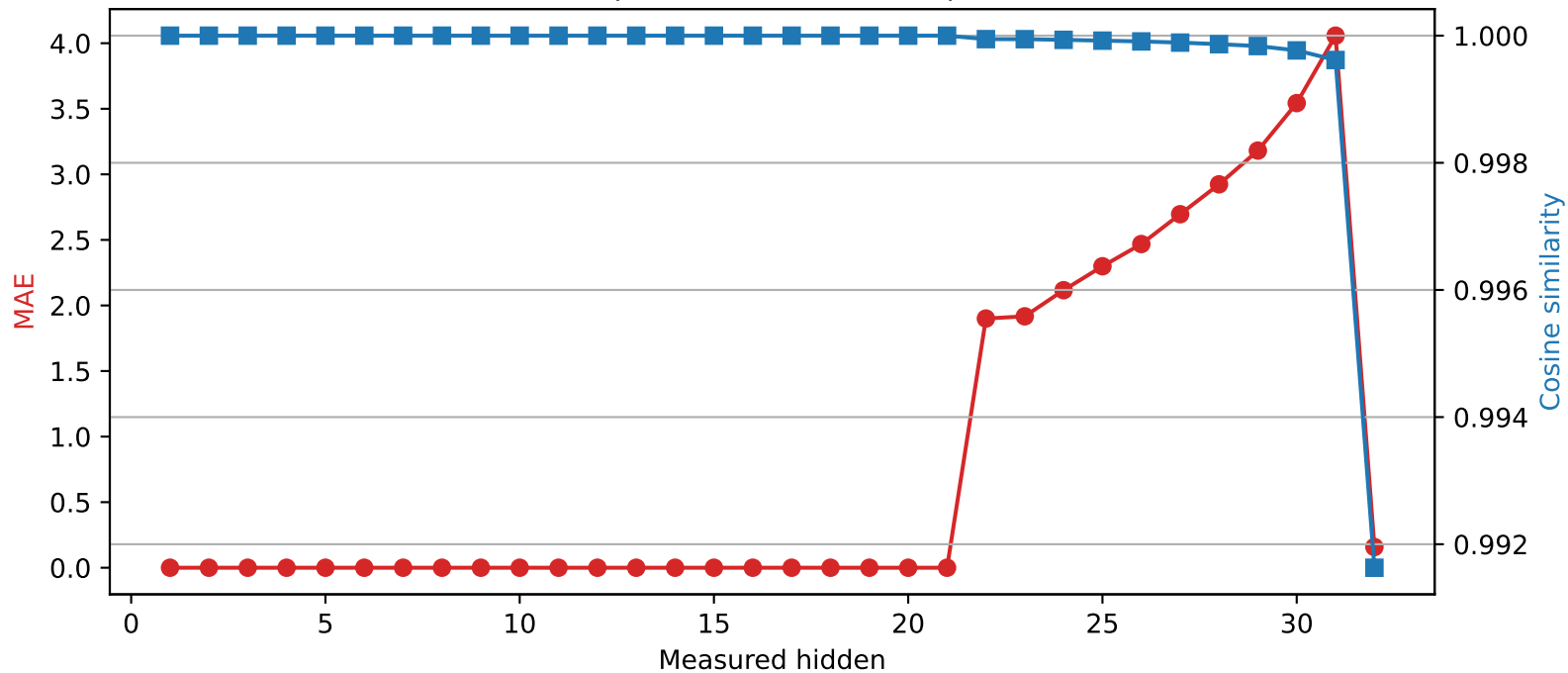
SmolLM2-360M | Quantized layer 21 | float64 → int4
