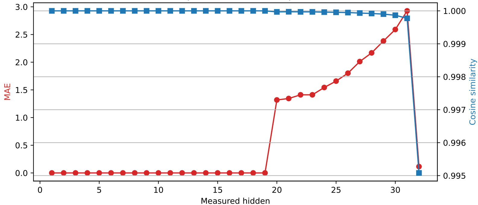
SmolLM2-360M | Quantized layer 19 | float64 → int4
