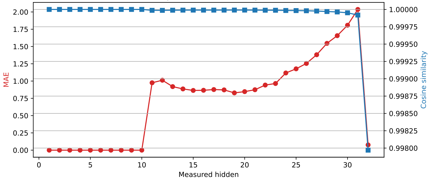
SmolLM2-360M | Quantized layer 10 | float64 → int4
