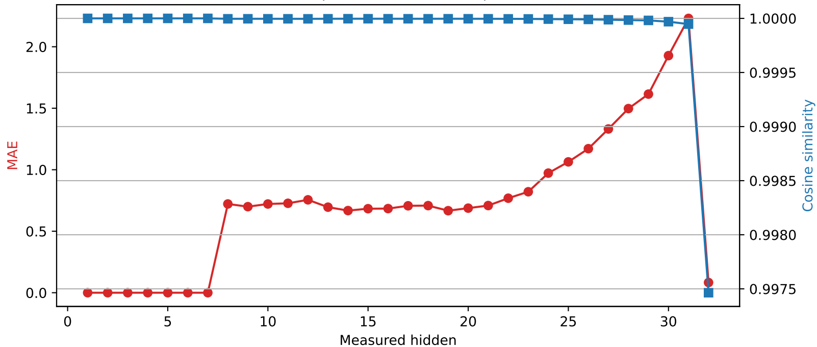
SmolLM2-360M | Quantized layer 7 | float16 \rightarrow int2
