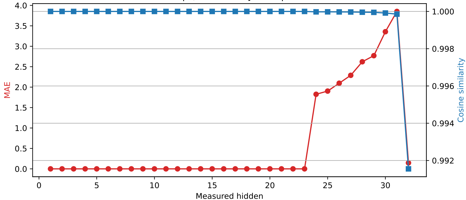
SmolLM2-360M | Quantized layer 23 | float16 \rightarrow int2
