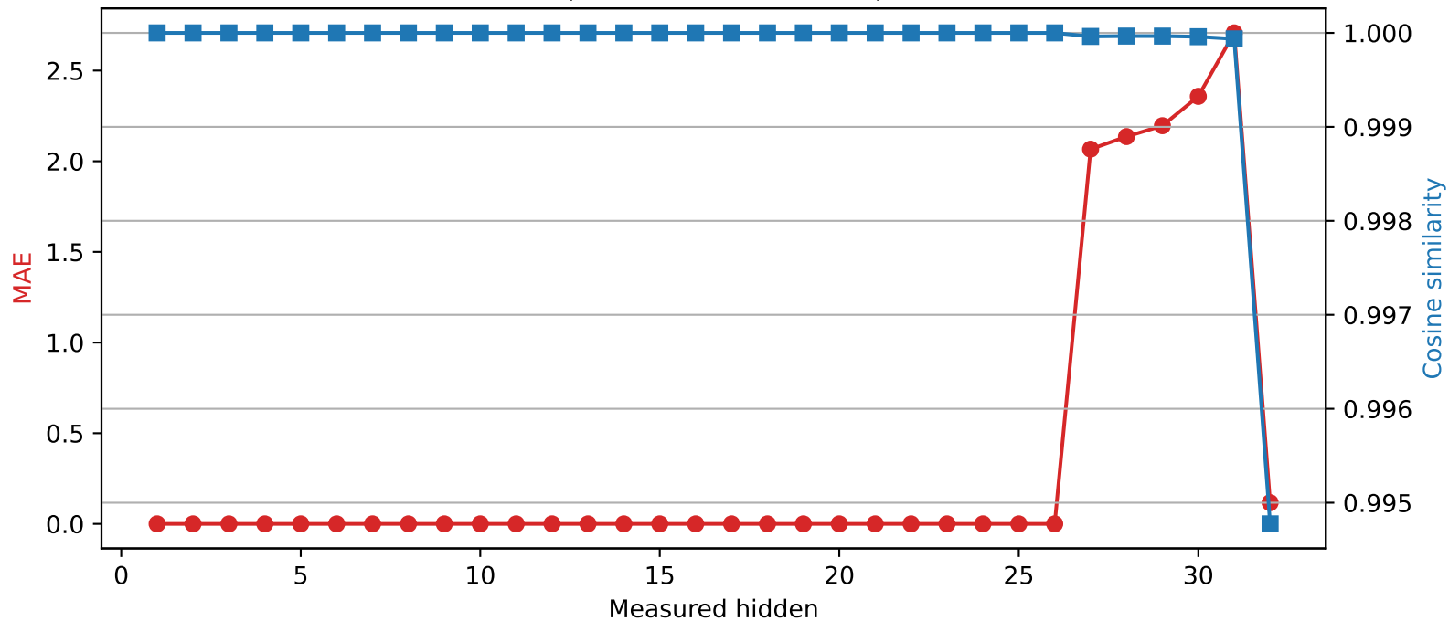
SmolLM2-360M | Quantized layer 26 | float16 \rightarrow int2
