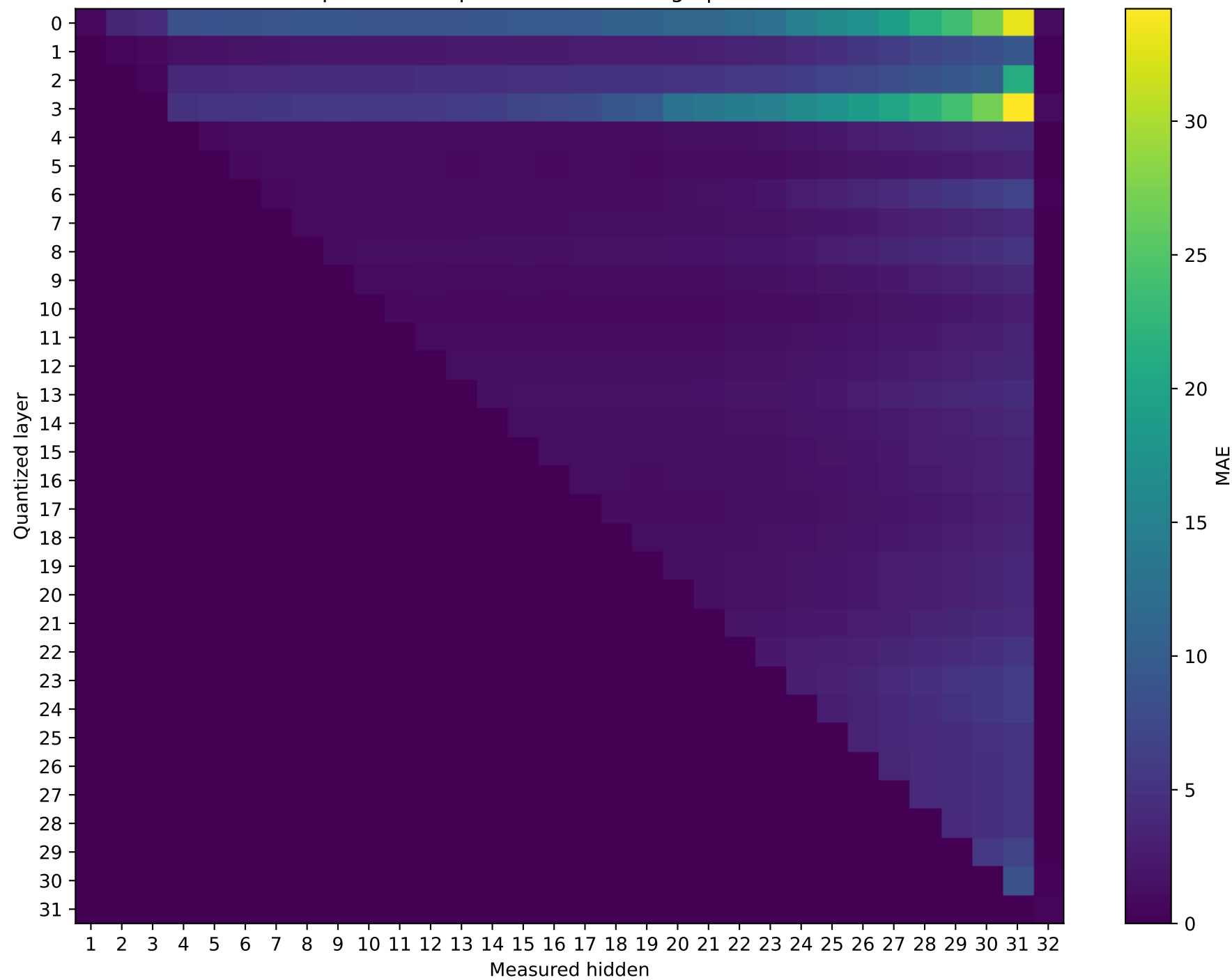
SmolLM2-360M Prompt 1: MAE representation damage | float16 \rightarrow int2
