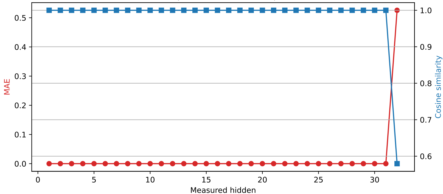
SmolLM2-360M | Quantized layer 31 | float16 \rightarrow int2
