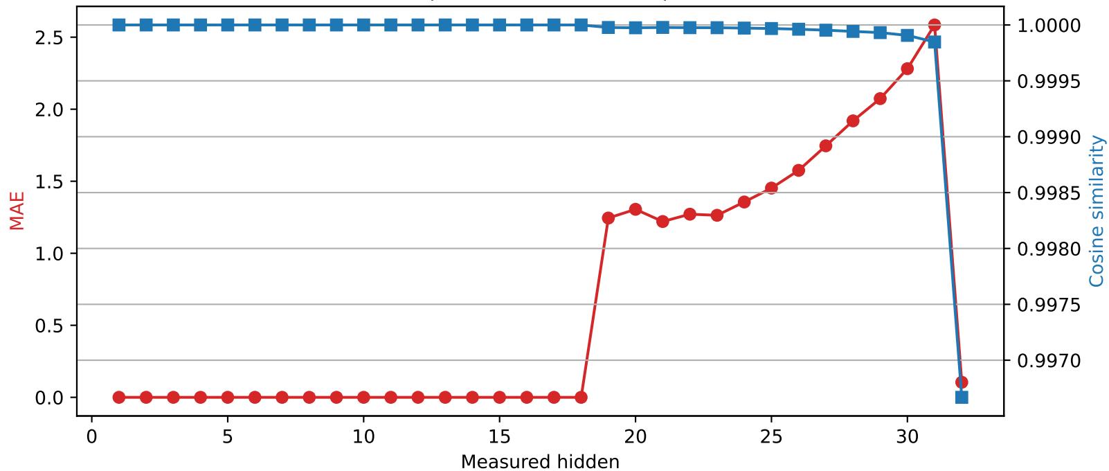
SmolLM2-360M | Quantized layer 18 | float16 \rightarrow int2
