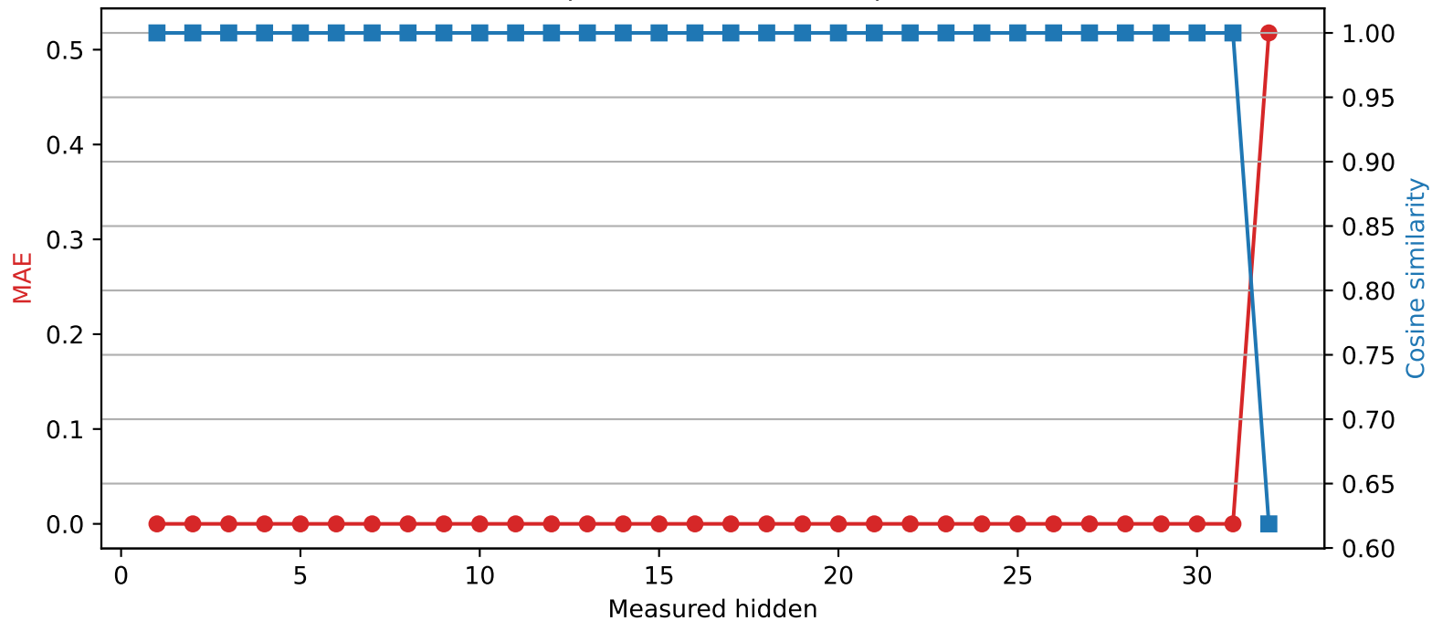
SmolLM2-360M | Quantized layer 31 | float16 → int2
