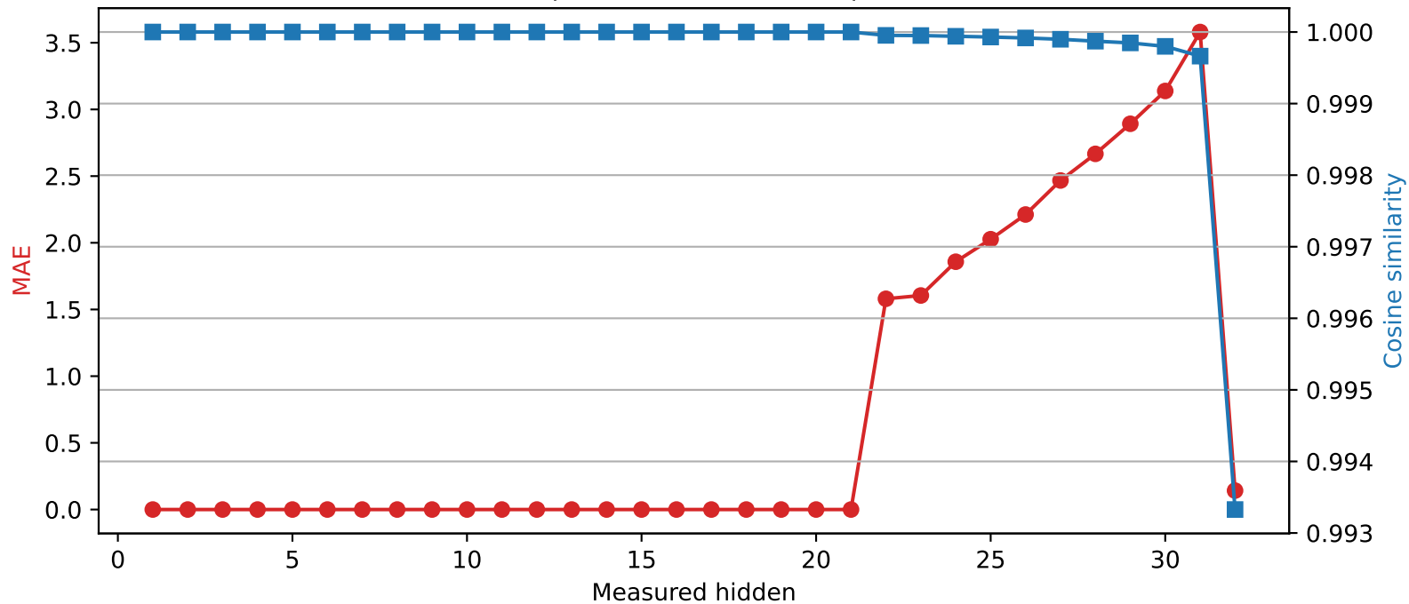
SmolLM2-360M | Quantized layer 21 | float16 → int2
