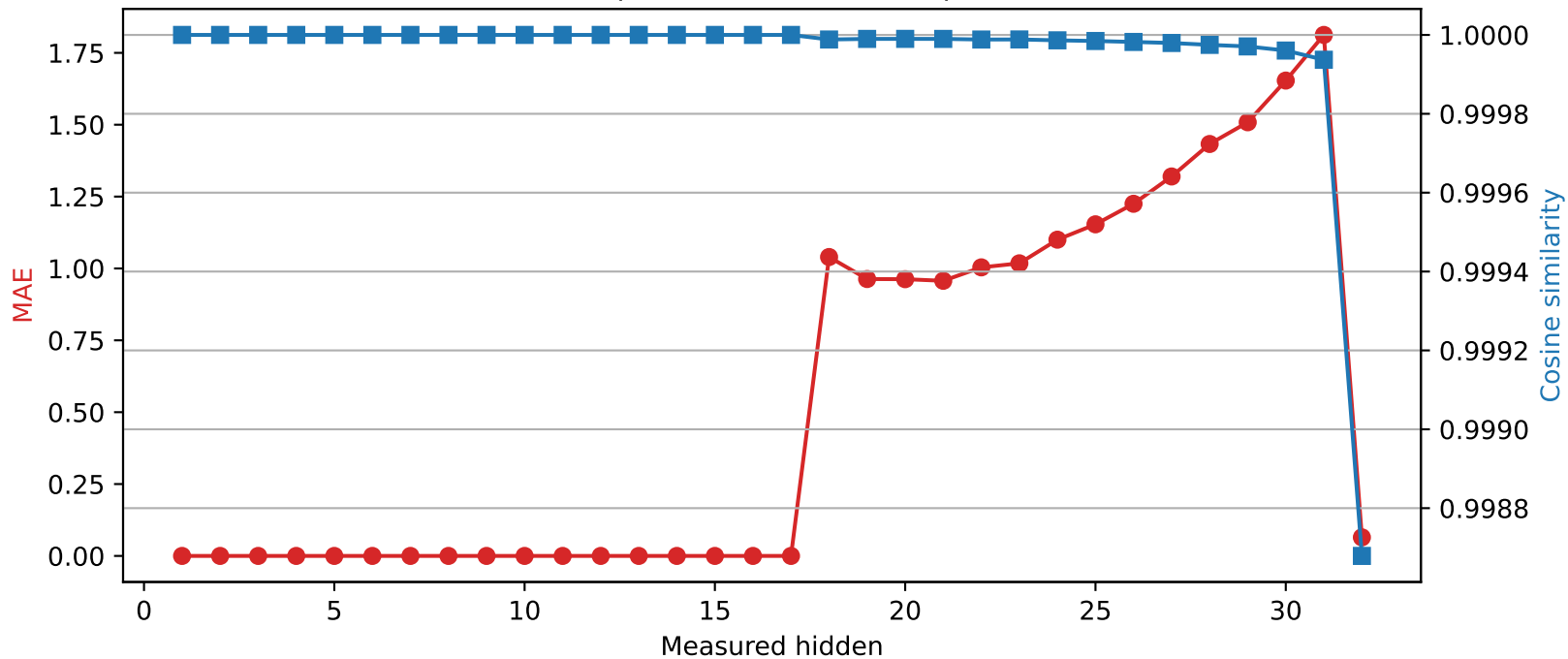
SmolLM2-360M | Quantized layer 17 | float16 → int2
