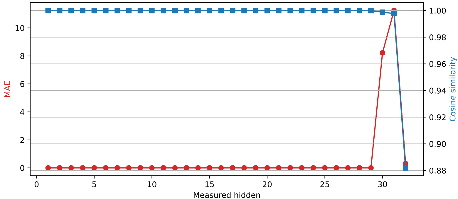
SmolLM2-360M | Quantized layer 29 | float32 → int2
