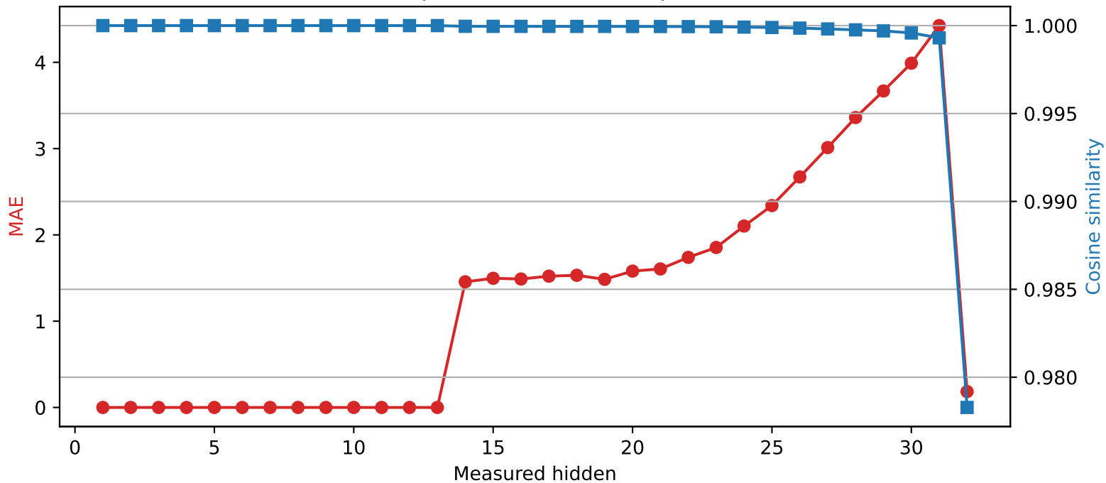
SmolLM2-360M | Quantized layer 13 | float32 → int2
