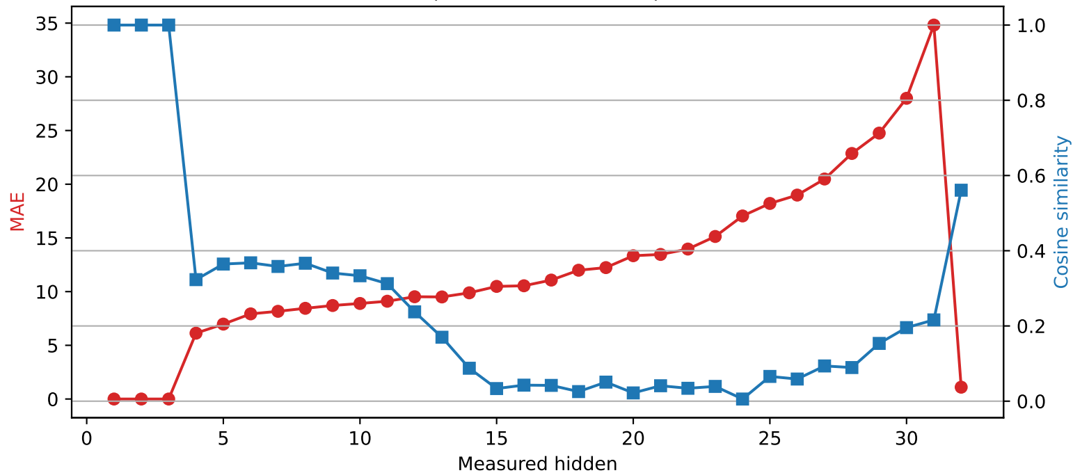
SmolLM2-360M | Quantized layer 3 | float32 → int2
