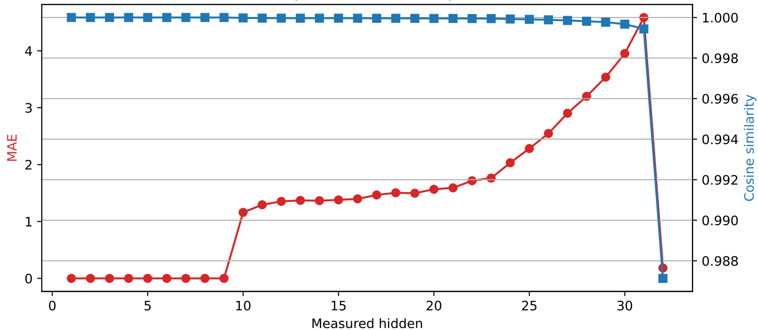
SmolLM2-360M | Quantized layer 9 | float32 → int2
