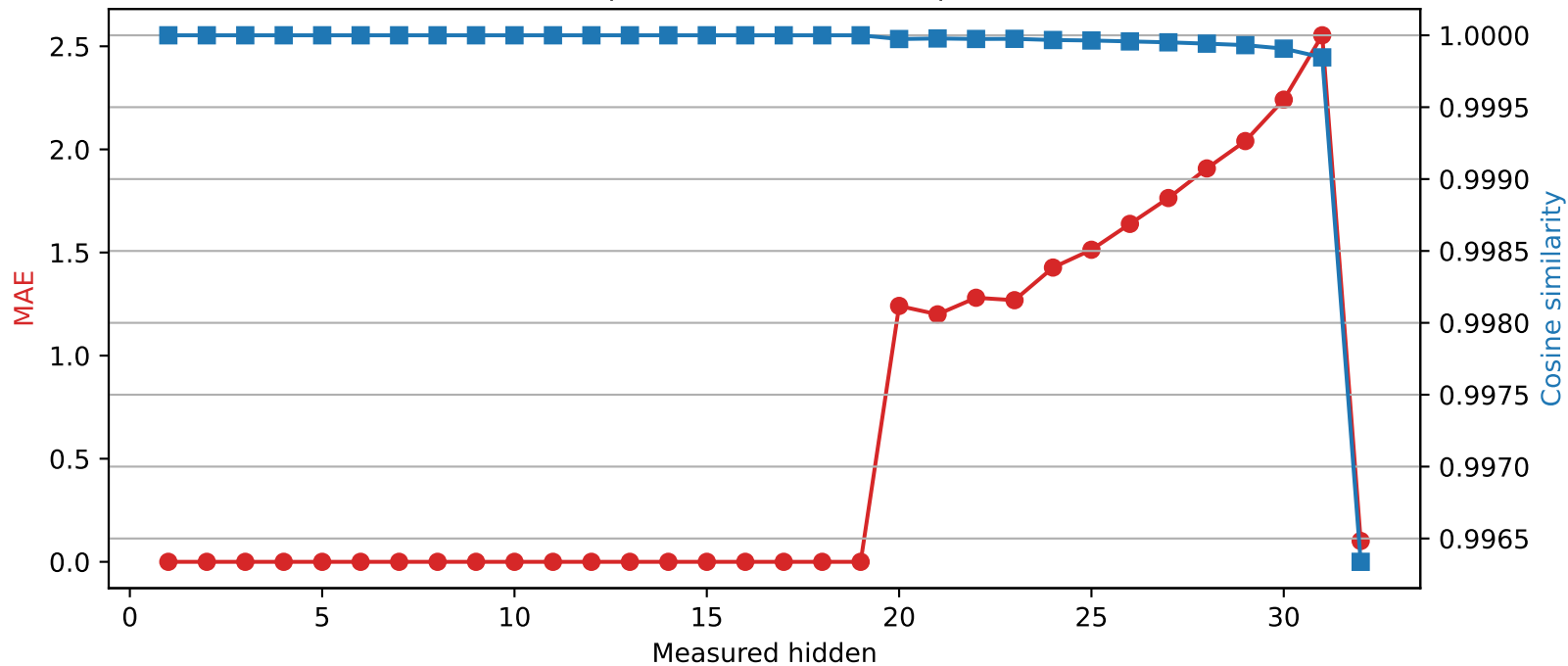
SmolLM2-360M | Quantized layer 19 | float32 → int2
