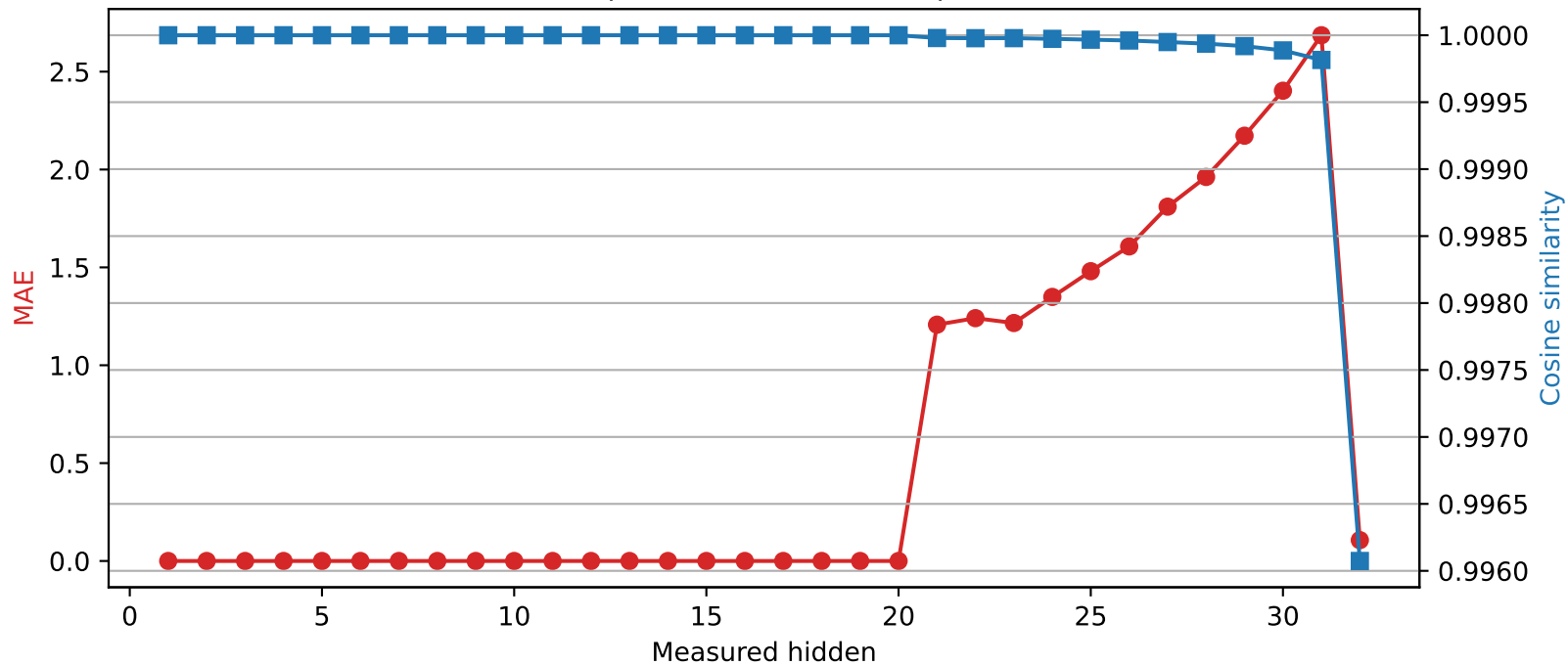
SmolLM2-360M | Quantized layer 20 | float32 → int2
