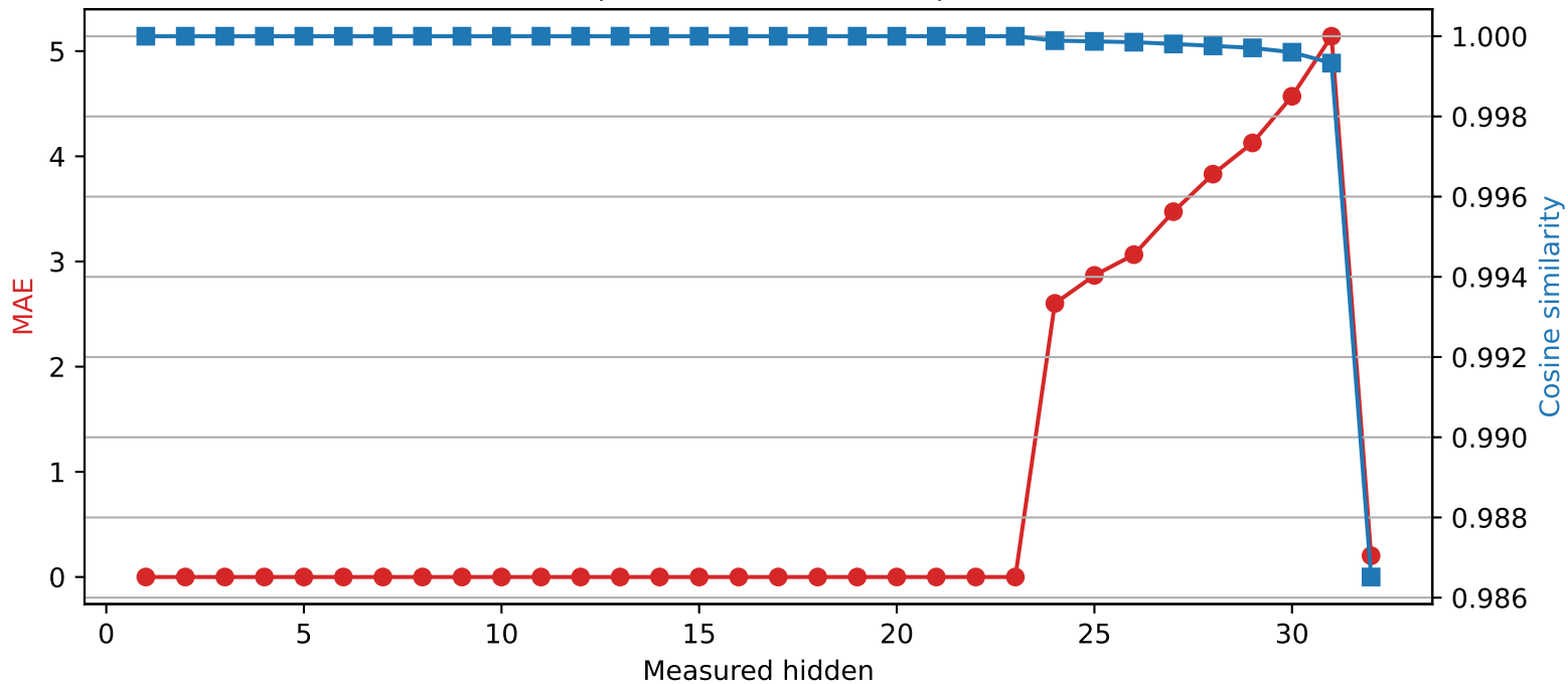
SmolLM2-360M | Quantized layer 23 | float32 → int2
