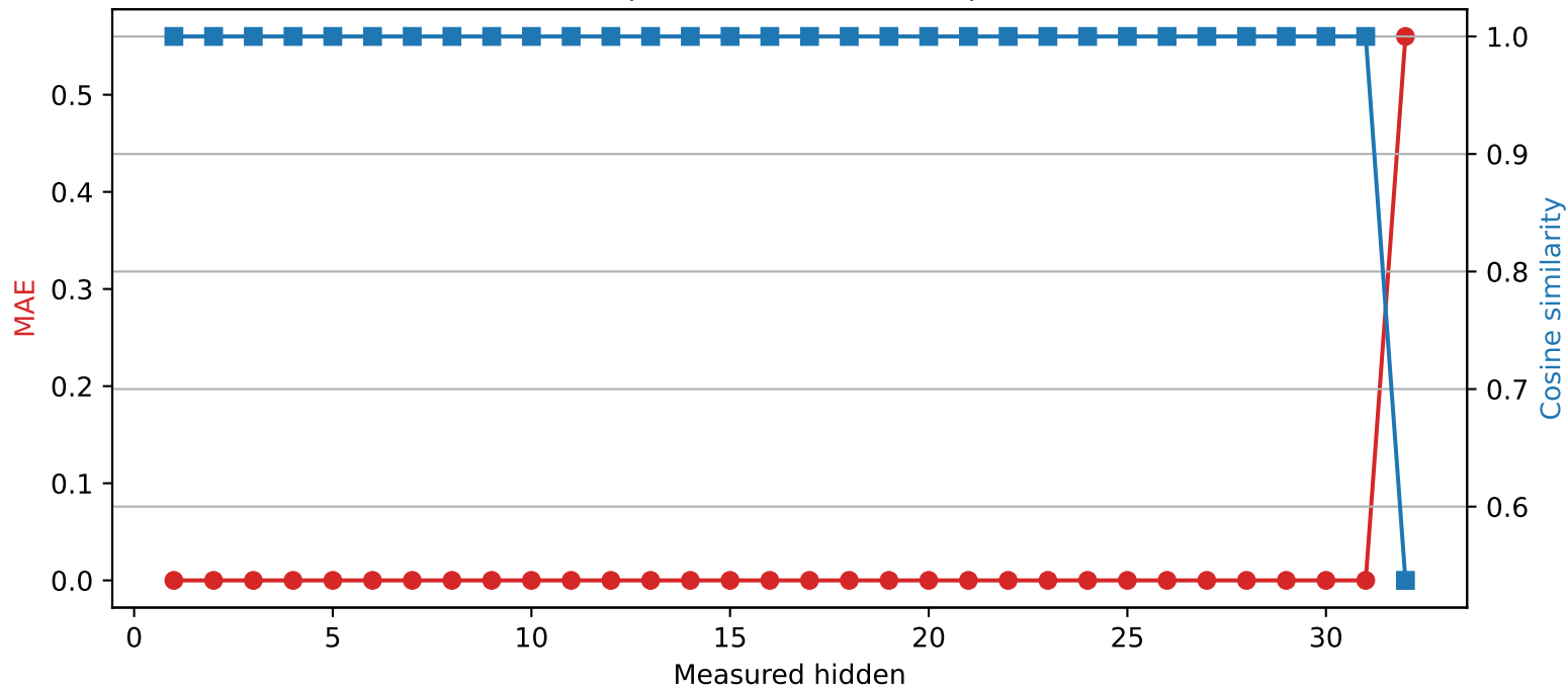
SmolLM2-360M | Quantized layer 31 | float32 \rightarrow int2
