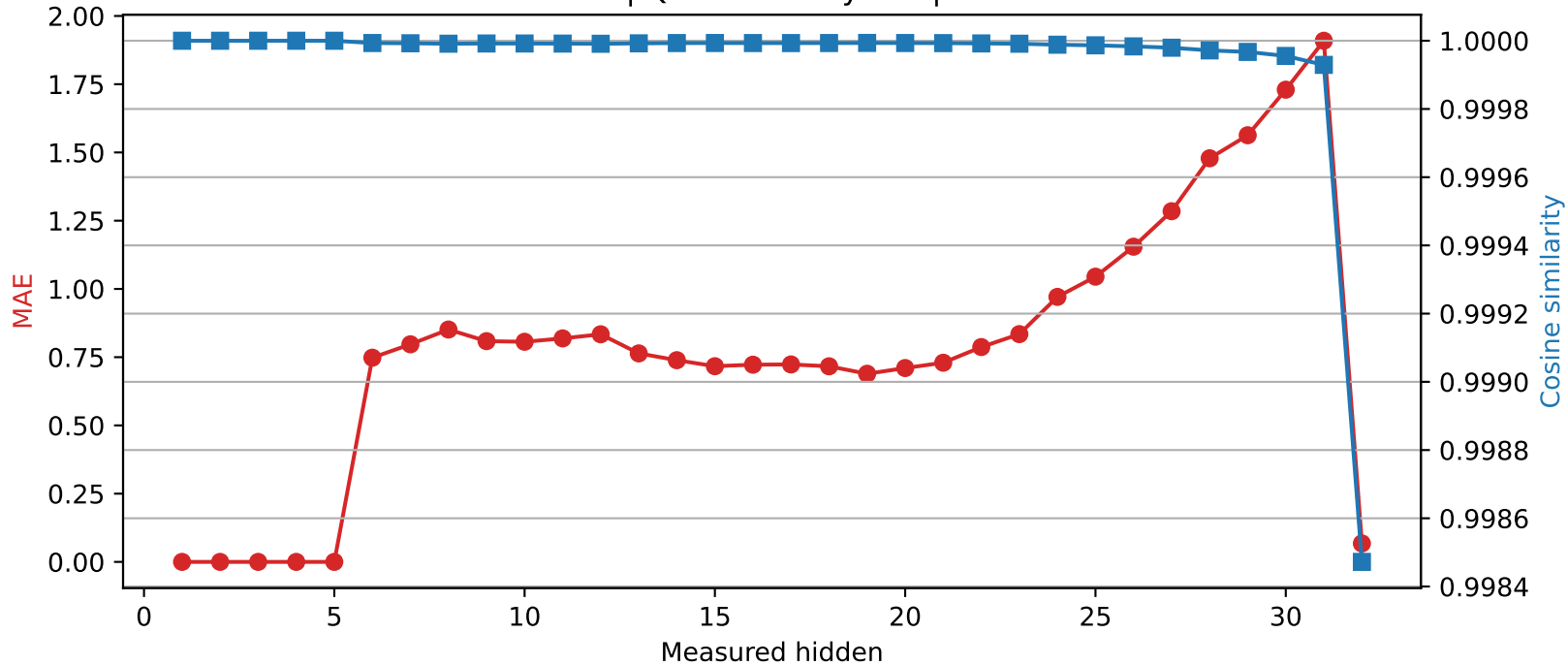
SmolLM2-360M | Quantized layer 5 | float32 → int2
