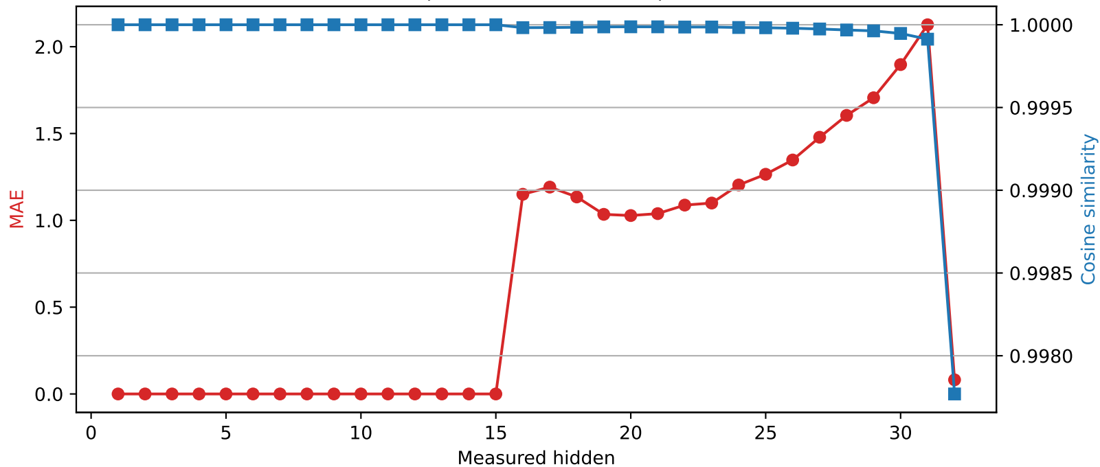
SmolLM2-360M | Quantized layer 15 | float32 → int2
