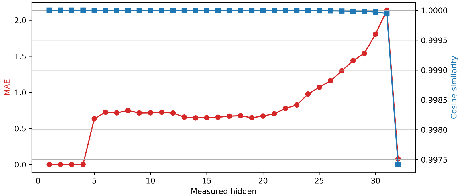
SmolLM2-360M | Quantized layer 4 | float64 → int2
