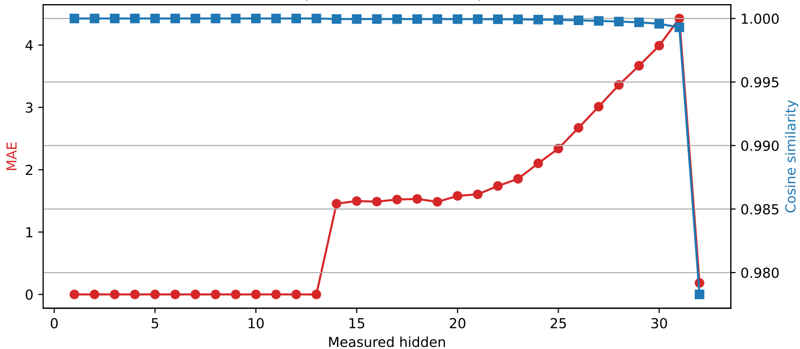
SmolLM2-360M | Quantized layer 13 | float64 → int2
