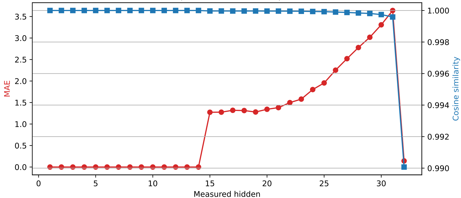
SmolLM2-360M | Quantized layer 14 | float64 → int2
