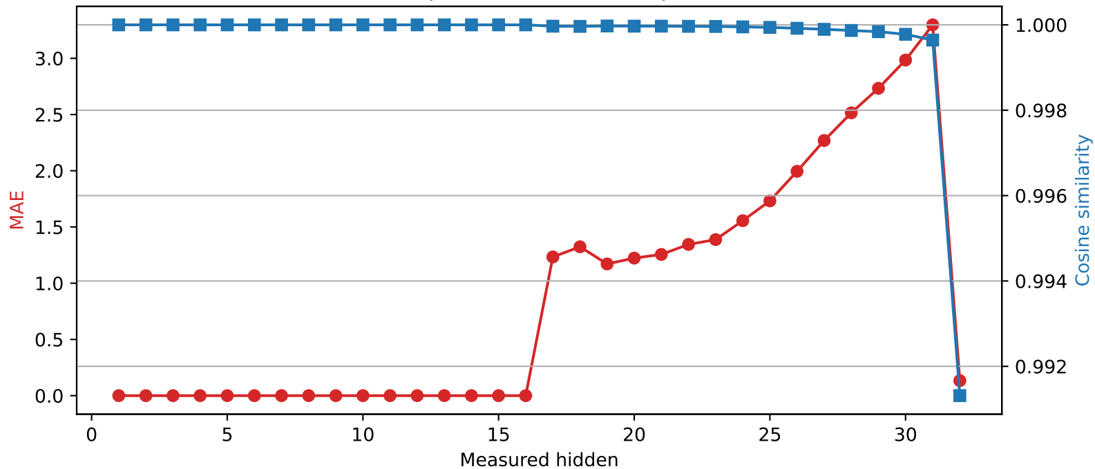
SmolLM2-360M | Quantized layer 16 | float64 → int2
